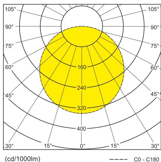
Photometric solid
