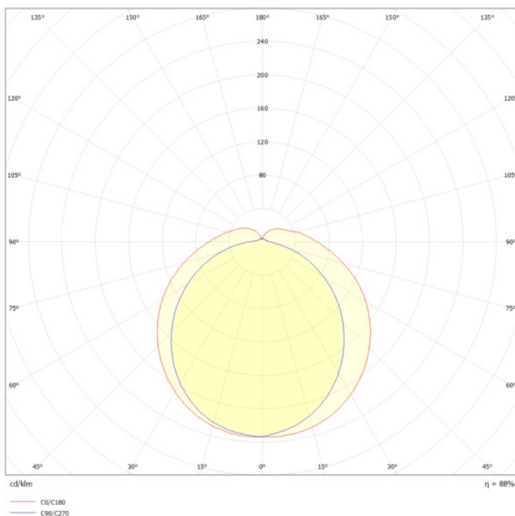
Photometric solid
